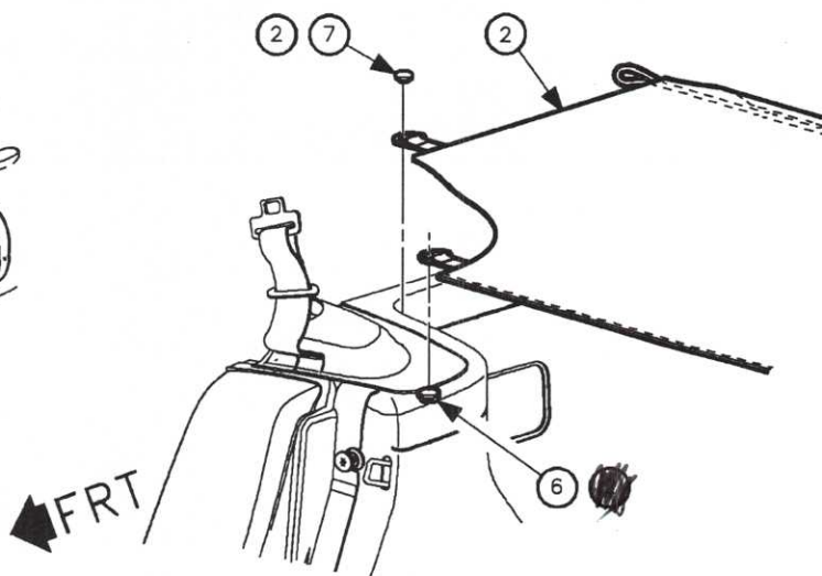
VIEW A RH SHOWN LH TYPICAL (1996-PRESENT)
